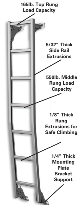
Universal Adjustable Mounting System fits to specific angle of roof
