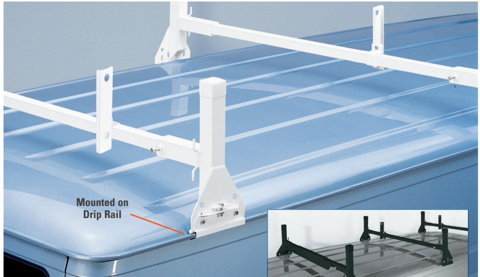
ULB-300 with optional Air Foil
