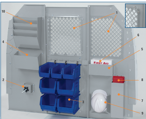
ProMaster, High Roof - Solid Partition
